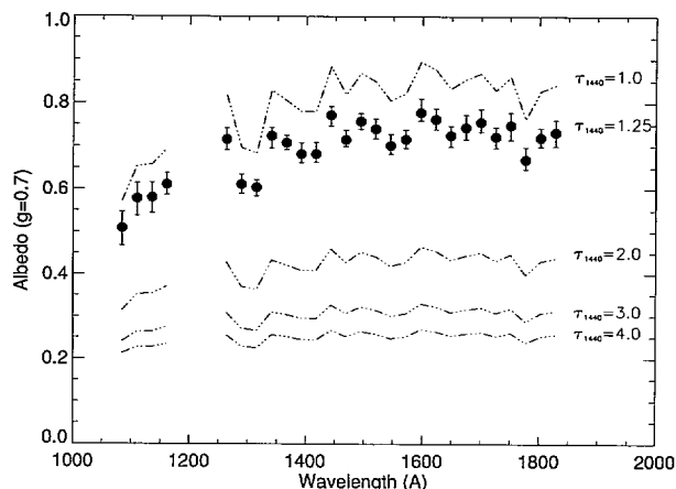
FIG. 3.—Albedo using E(B - V) = 0.14 in the nebula (the value assumed by Witt et al. 1982, 1992) plotted as filled circles with \pm 1 \sigma error bars. The spectra of Fig. 1 have been binned in groups of 50 to increase the signal-to-noise ratio. Also shown are a number of other models (dashed lines) corresponding to different amounts of extinction in the nebula. We have calculated these albedos assuming spherical models of the appropriate column density in front of the star. Although the IR constraints rule out these specific models, hemispherical models of the same optical depth (in front of the star) may be allowed (see text).
