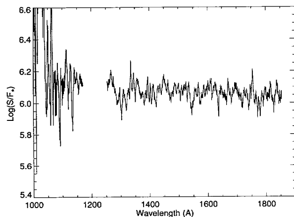
FIG. 2.—Logarithm of the ratio of the nebular surface brightness ( S ) at the location of the HUT 18'' aperture to the stellar flux ( F_* ) smoothed over 5 bins. The region around Ly \alpha is dominated by the geocoronal line and has been excised. There is too little flux below about 1100 \text{ \AA} to allow the data to be used. The main observational result of this paper is the constancy of the ratio S/F_* .
