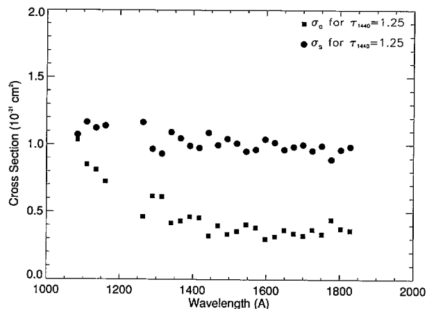
FIG. 4.—Cross sections for absorption ( \sigma_a ) and scattering ( \sigma_s ) are plotted for E(B - V) = 0.14 ; \sigma_a shows a sharp increase toward shorter wavelengths, implying that much of the FUV rise in the extinction curve must be due to an increase in absorption.
