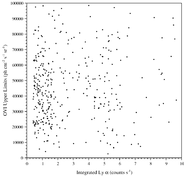
FIG. 1.—Derived O VI upper limits plotted against the integrated counts in the Ly \alpha line. There is no correlation between the two. Such a correlation might be expected if systematic errors were an important contributor to the O VI limits. Similar plots are obtained when the O VI limits are plotted against the relative RTG strength or the diffuse continuum; none of the different components are correlated, indicating that systematic errors are unimportant in our analysis.
