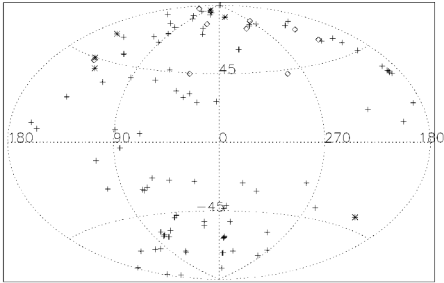
Fig. 2.—All of the Voyager observations for which we were able to set upper limits of less than 5 \times 10^{-7} ergs \text{cm}^{-2} \text{sr}^{-1} \text{s}^{-1} ( 25,000 photons \text{cm}^{-2} \text{sr}^{-1} \text{s}^{-1} ) are plotted as plus signs on an Aitoff map of the sky, with the origin at the center and 180^\circ at the left. The Dixon et al. (1996) targets are plotted as diamonds, and the C IV detections of Martin & Bowyer (1990) are plotted as asterisks. In one direction in common (see text), we place a 90% confidence limit that is about half the claimed detection by Dixon et al.; however, given both sets of uncertainties and the different locations, we cannot rule out their claimed value.
